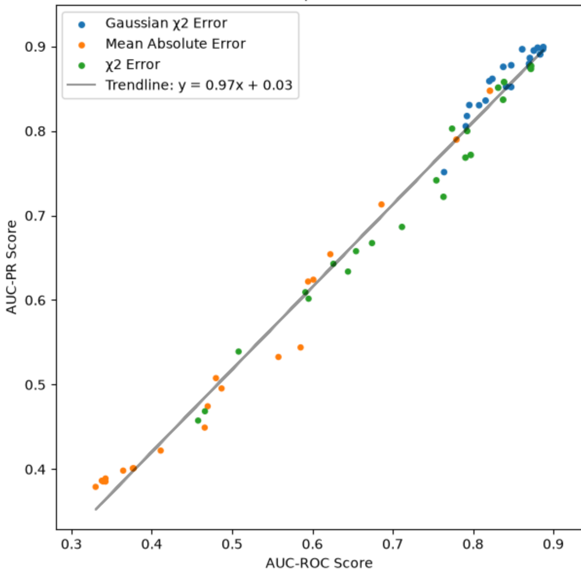
AUC Scatterplot (Loss View)
